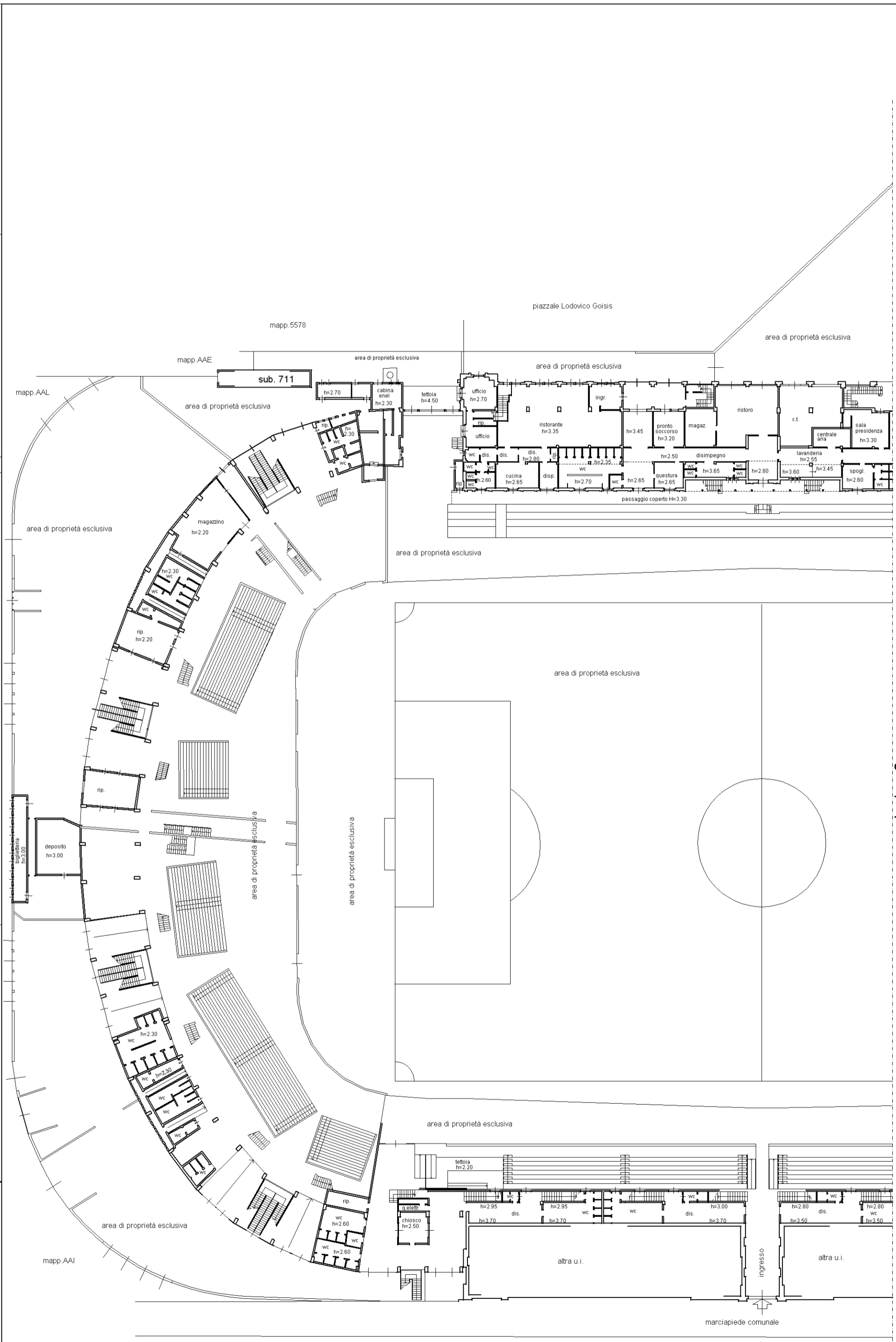
PIANO TERRA
